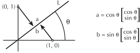
Fig. 2.2. Projection of unit coordinates (1,0) and (0,1) onto line L , which is inclined by angle \theta and passes through the origin. The projected coordinates are tabulated on the right. A second projection of a and b onto L does not change the coordinates of a and b . The projection operator is non-invertable.
