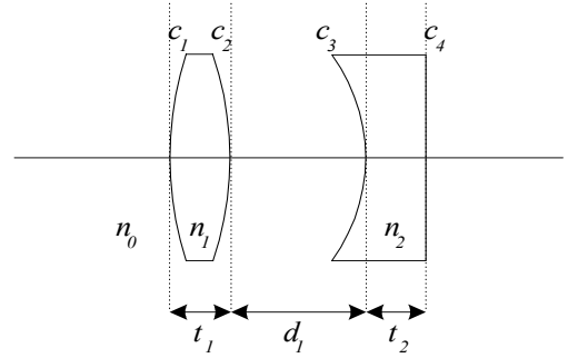
Figure 1: Parameters of a Two Lenses System. The n_i variables denote the refractive indexes of the media, the c_i represent the lens surface curvatures, the t_i are the lens thicknesses, and d_1 is the lens spacing.
