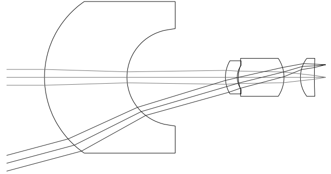
Figure 6: Best Design Found with GA
