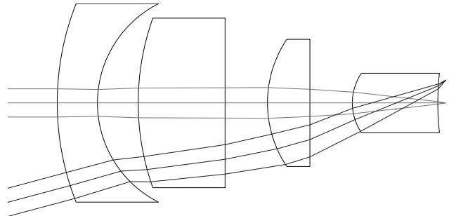
Figure 8: Best Design Found with GP (Using the Raw System as Starting Point)
