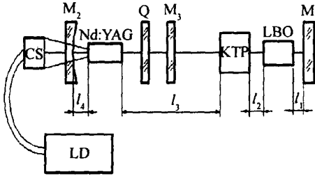
Fig 2 LD pumped ultraviolet laser
