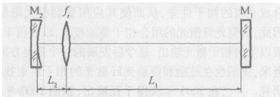
Fig 3 Equivalent resonator schematic
