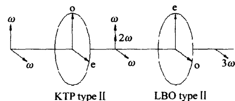
Fig 1 Light polarizing match in KTP and LBO
