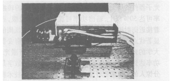
Fig 4 LD pumped 355nm quasi-CW ultraviolet laser
