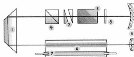
1) folding prism; 2) alignment prism; 3) KD*P crystal; 4) cube polarizer; 5) resonator mirrors; 6) Nd:YAG rod; 7) flashlamp; 8) quarter waveplate
