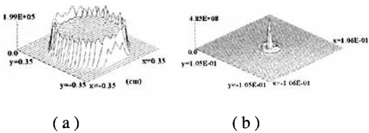
Fig.2 (a) near-field and (b) far-field energy profile at pass 30 corresponding to 60 ns
