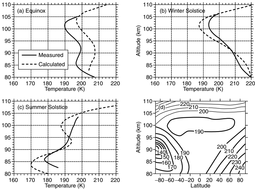
Fig. 11.10. Calculated and measured nighttime averaged temperature profiles over Fort Collins, CO (41°N, 105°W) for (a) equinox, (b) winter, (c) summer, along with calculated altitude-latitude plots of zonal mean temperature contours in the mesopause region for December solstice solar cycle minimum geomagnetic quiet conditions, in (d). From She et al. [52].
