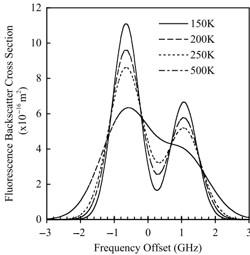
Fig. 11.7. Na D 2 Doppler-broadened fluorescence spectrum plotted as a function of frequency for four temperatures.
