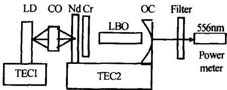
图 2 556 nm 脉冲激光器实验原理图 Fig. 2 The schematic diagram of pulse laser at 556 nm
