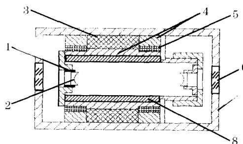
Fig. 1. Schematic configuration of F-P cavity for temperature control. 1: PZT; 2: cavity mirror; 3: bakelite sheath; 4: copper sheath; 5: TEC modules; 6: transparency window; 7: aluminum box; 8: invar tube.
