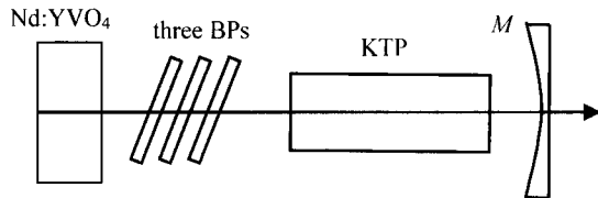
Fig. 3. A resonator with three Brewster plates.
