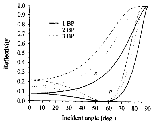
Fig. 1. Reflectivity loss of multi-Brewster plates vs. incident angle.
