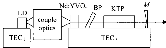
Fig. 2. A laser resonator with a Brewster plate.
