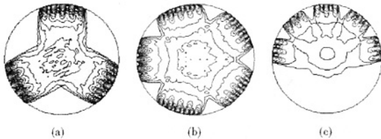
图 10 多侧面泵浦晶体的泵浦光强等高线分布示意图 Fig.10 Calculated pumping energy distribution contour for multi-sided pumping configuration
