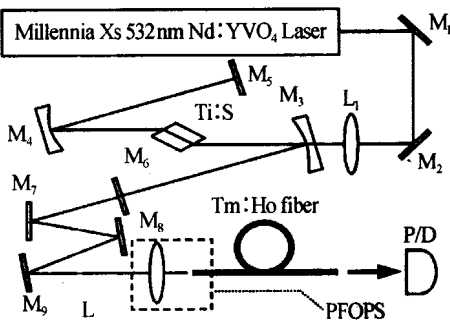
图 2 钛宝石泵浦 Tm2Ho 共掺石英光纤激光器的实验装置 Fig. 2 Schematic diagram of the experimental setup of the Ti:S pumped Tm2Ho co-doped silica fiber laser
