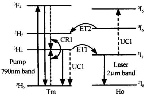
图 1 Tm2Ho 共掺石英光纤系统能级结构 Fig. 1 Schematical energy level diagram of Tm2Ho co-doped silica fiber system
