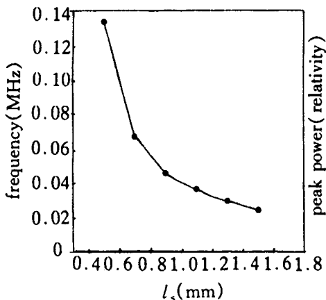
Fig. 7 The influence of the length of the \text{Cr}^{4+} YAG to the pulse frequency
