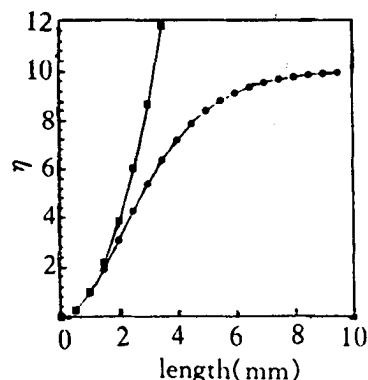
Fig. 3 Comparison of the doubling efficiency of small signal and high signal
