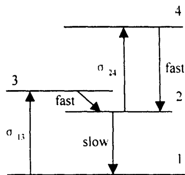
Fig. 1 The 4-level model of Cr 4+ 2doped saturable absorber
