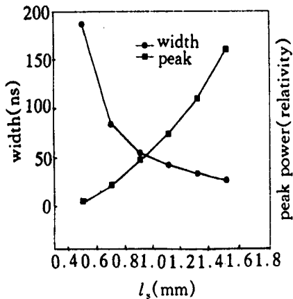
Fig. 8 The influence of the length of the \text{Cr}^{4+} YAG to the pulse width and peak power
