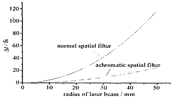
Fig. 5 Propagation time delay of different spatial filters
