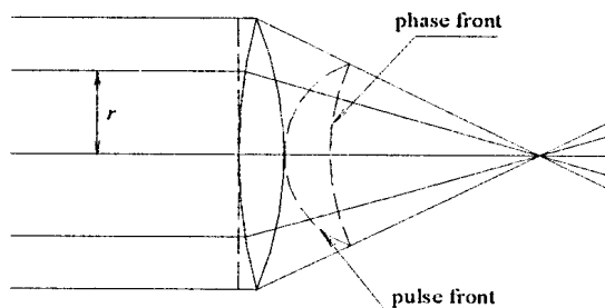
Fig. 1 Temporal front of the laser pulse delayed with respect to the phase front
