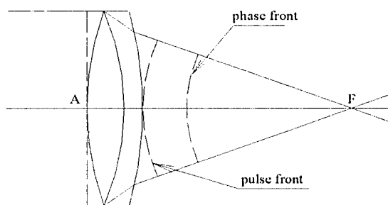
Fig. 3 Delay between the phase and pulse front
