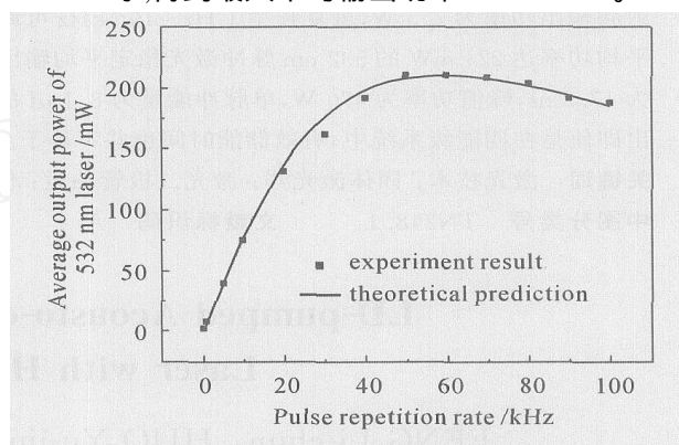
图 2 532 nm 激光输出平均功率随脉冲重复频率的变化 Fig. 2 Average output power of 532 nm laser as a function of the Q -switched pulse repetition rate
