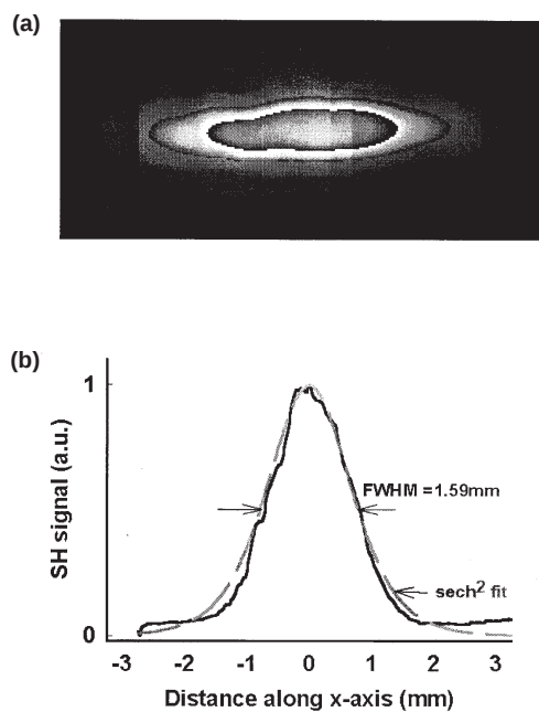
Figure 3. (a) CCD image of the SH signal (autocorrelation) generated in the KDP crystal. (b) Spatial intensity profile ( x -direction) of the SH beam. FWHM of the distribution (1.59 mm) corresponds to a laser pulse duration of 250 fs (taking correction factor for input intensity variation across the input beam diameter). Dotted line shows the calculated auto-correlation function for a \text{sech}^2 shaped laser pulse of 250 fs (FWHM) duration.
