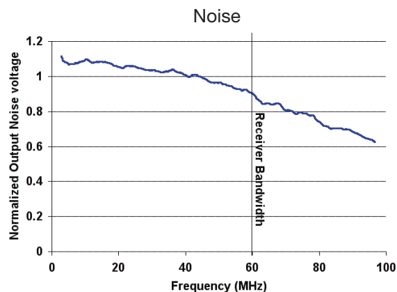
Figure 4. Typical Response / Noise Curves
