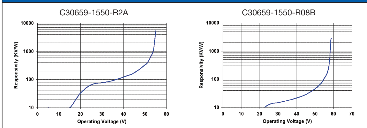
Figure 4. Typical Response / Noise Curves
