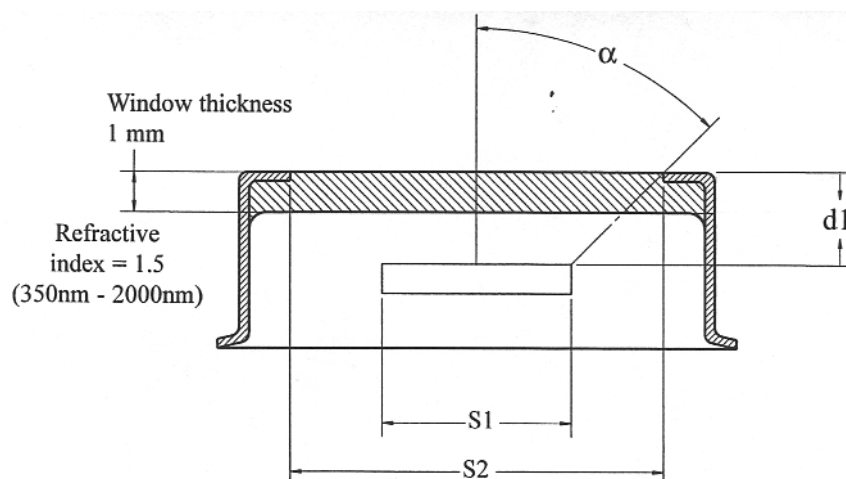
Figure 6. Optical Geometry
