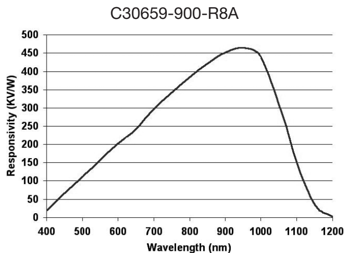
Figure 2. Spectral Responsivity
