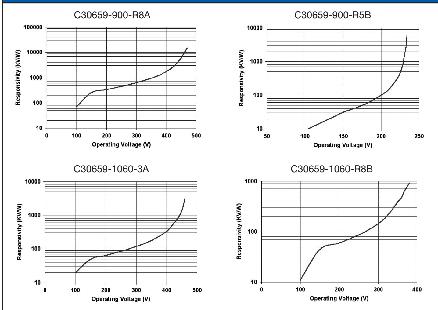
Figure 3. Responsivity
