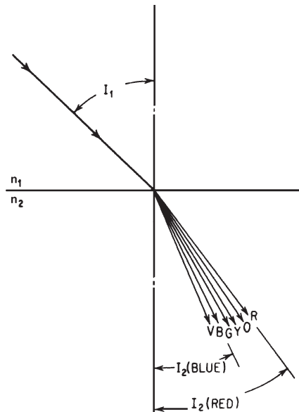
Figure 1.6 Showing the dispersion of white light into its constituent colors by refraction (exaggerated for clarity).
