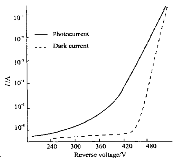
图 1 Si-APD 器件的伏安特性曲线 Fig. 1 V-I characteristics of Si-APD devices
