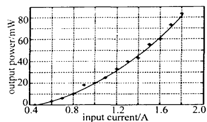
Fig 2 SFM 593.5nm output power via input current
