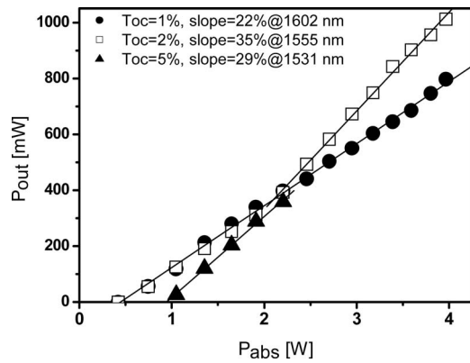
Fig. 5. Input–output characteristics of CW Er,Yb:YAB laser.
