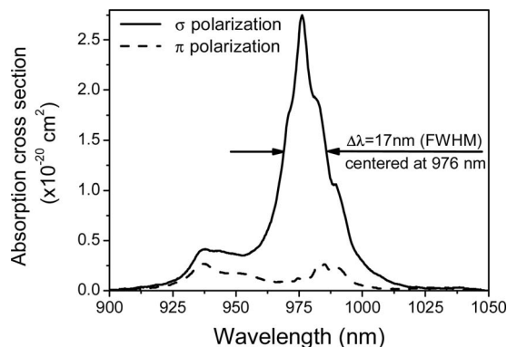
Fig. 1. Room-temperature polarized absorption spectra of Er, Yb:YAB crystal at 1 μm.
