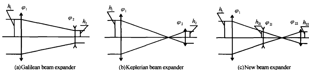
图1 扩束器类型 Fig.1 Optical systems of beam expanders
