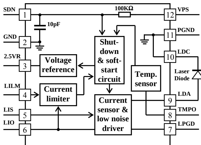
Figure 3 Block Diagram
