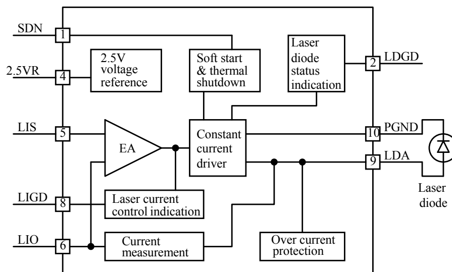
Figure 3 Block Diagram
