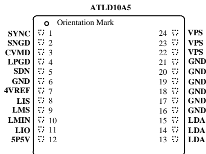
Figure 1 Top View of ATLD10A5
