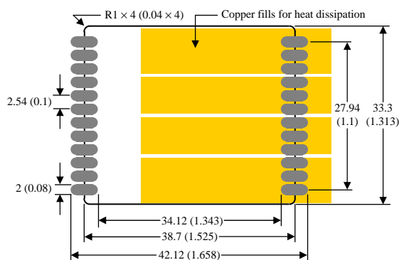
Figure 6 Recommended Foot-print for the SMT Package
