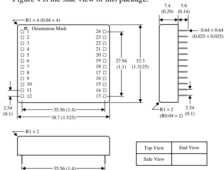
Figure 4 Mechanical Drawings for ATLD10A5-D
