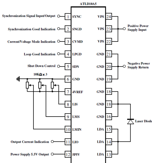
Figure 2 Typical Application Connection
