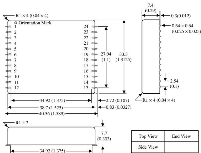
Figure 5 Mechanical Drawings for ATLD10A5-S
