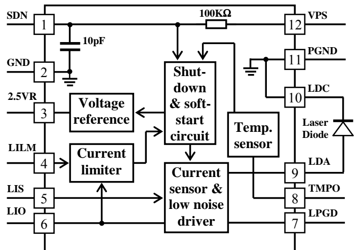
Figure 3 Block Diagram
