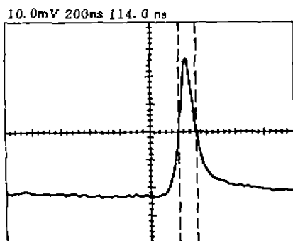
Fig. 3 Oscilloscope trace of a typical laser pulse from the passively Q -switched 1064 nm Nd:YVO 4 laser with a 500 mW pump power. The horizontal scale is 200 ns/div. The two dashed lines mark the pulse width of 114 ns
