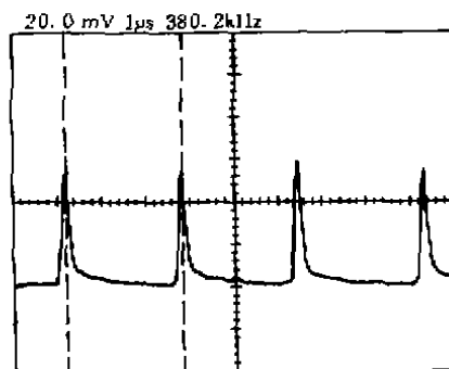
Fig. 4 A typical sequence of laser pulses from the passively Q -switched 1064 nm Nd:YVO 4 laser with 500 mW of pump power. The horizontal scale is 1 μs/div. The two vertical dashed lines mark the pulse period of 2.63 μs which corresponds to a pulse repetition rate of 380.23 kHz
