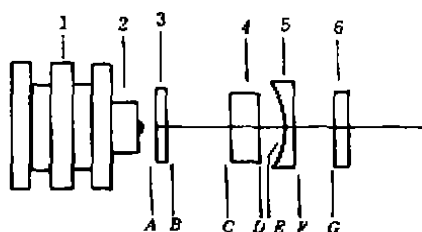
Fig. 1 Diagram of the passively Q -switched Nd:YVO 4 laser pumped by a laser diode. The schematic of direct-coupled pump (DCP) is used
