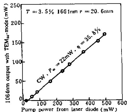
Fig. 2 Output power of the CW 1064 nm Nd:YVO 4 laser versus the pump power of the laser diode
