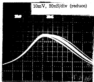
Fig. 4 A multiple exposure of 50 output pulse with negative feedback control (20 ns, 10 mV/div)
