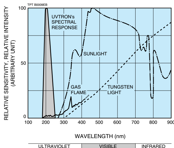
Figure: UVTRON's Spectral Response and Various Light Sources
