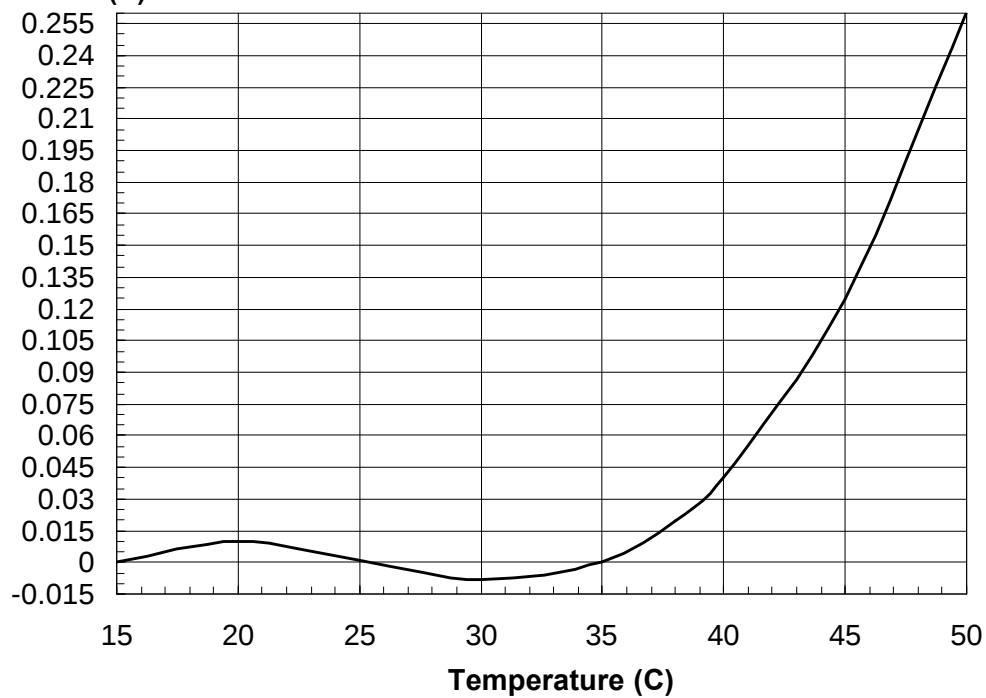
Linearity Error in TEMPSP v.s. Temperature
