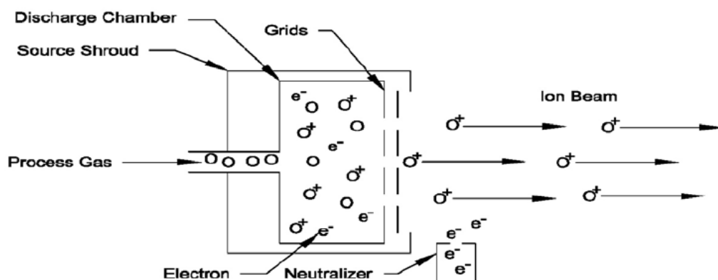
Figure 1. Schematic of an Ion Beam Source
