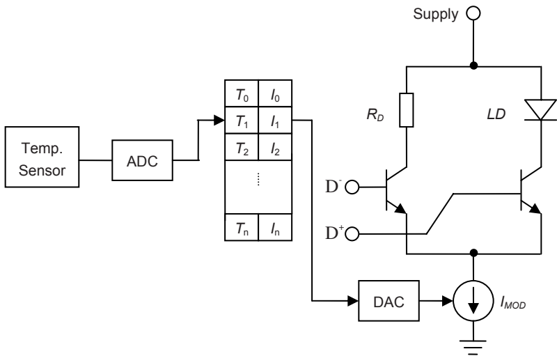
Fig. 8.11. Look-up table scheme for modulation control
