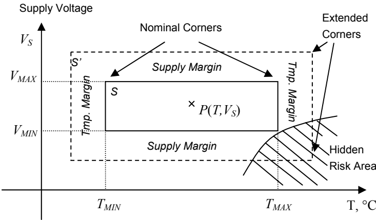
Fig. 10.4. Sample parameter space for an optical transmitter
