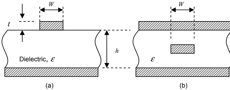
Fig. 3.8. (a) Microstrip and (b) stripline transmission lines
