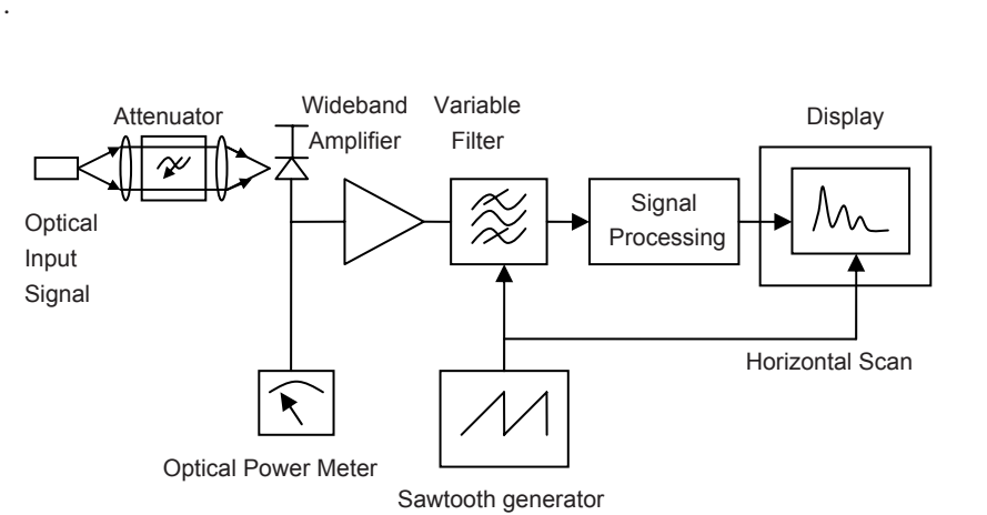
Fig. 11.13. Principals of operation of a lightwave signal analyzer (LSA)
