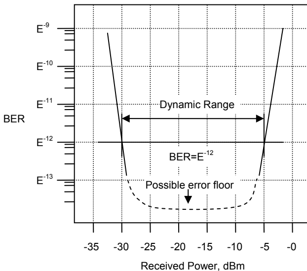
Fig. 9.14. Representative behavior of a receiver from sensitivity to overload
