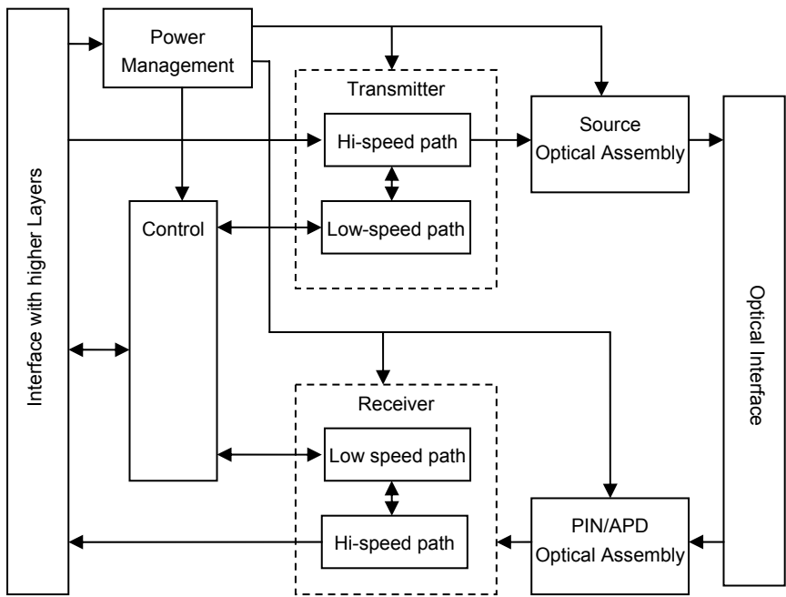
Fig. 10.2. Physical layer building block and functional interconnections
