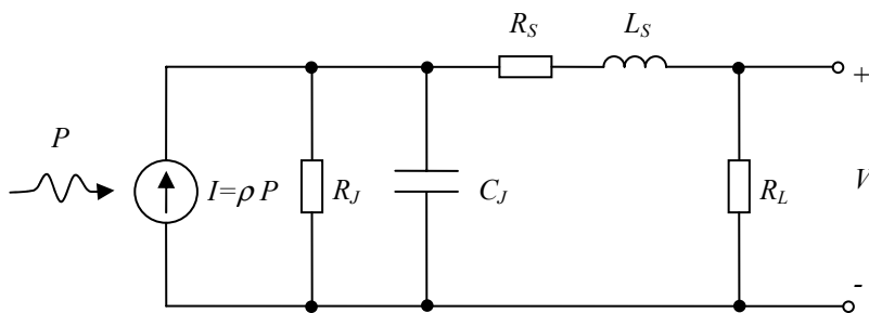
Fig. 6.4. ac model of a PIN detector
