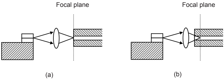
Fig. 10.7. Sensitivity of coupling efficiency to optical alignment. (a) focal imaging, (b) out of focus imaging
