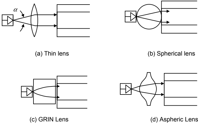
Fig. 7.3. Commonly used lens structures to improve coupling efficiency
