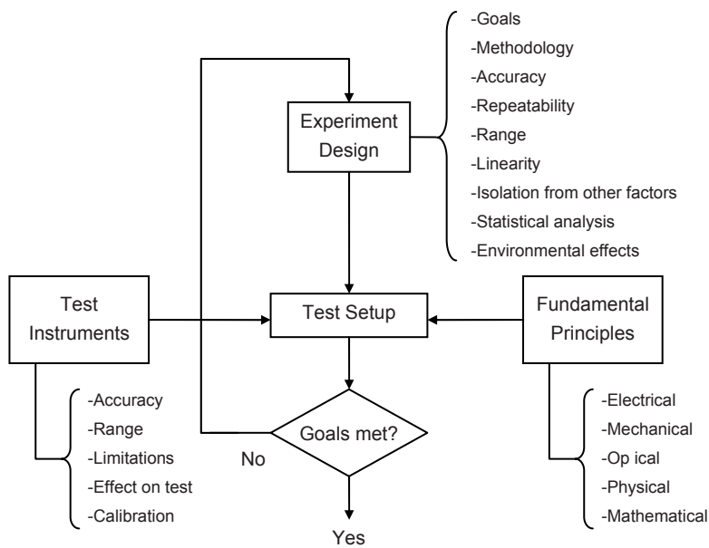
Fig. 11.1. Elements of a measurement experiment
