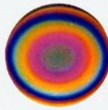
附图 8 N = -1.7 \quad \Delta_1 N = 0.3
