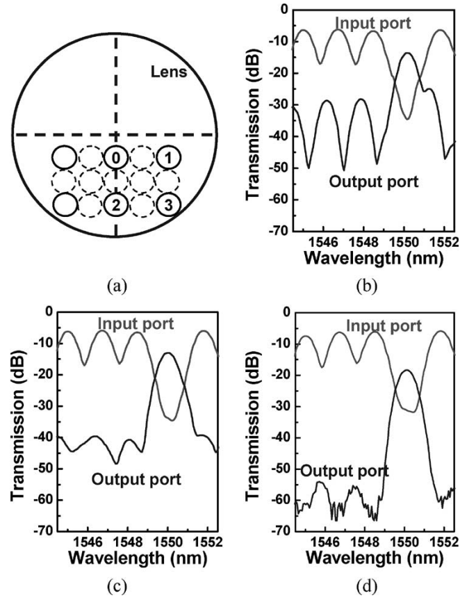
Fig. 10. (a) Cross-section of the 1 \times N^2 WSS. Port 0 is the input, while the other ports are serving as the outputs. (b)–(d) Spectra when the 1550-nm wavelength channel is switched to ports 1, 2, and 3, respectively. Five wavelength channels are shown.
