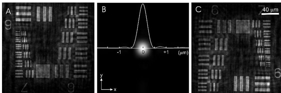
Fig. 6. A, Twin image of C (i.e., reconstructed at the same distance on the other side of the pinhole); B, reconstruction at the origin, showing the pinhole of size 0.5 \mu\text{m} .
