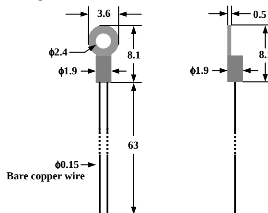
Figure 1 The Front and Side Views of ATH10KL2A
