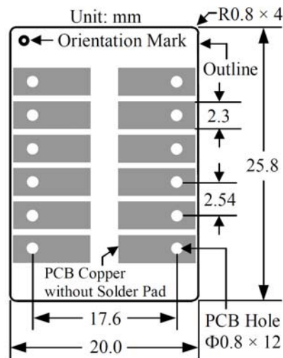
Figure 10. Top View of the Top Side PCB Foot-print
