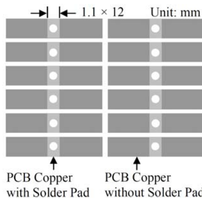
Figure 11. Top View of the Bottom Side PCB Foot-print
