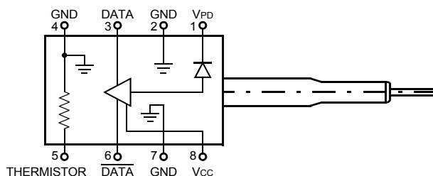
Figure 1. P172-Type Receiver (Top View)
