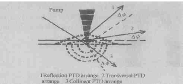
图 1 光热偏转效应和检测方式 Fig. 1 Diagram of photothermal deflection effect and detection arrange
