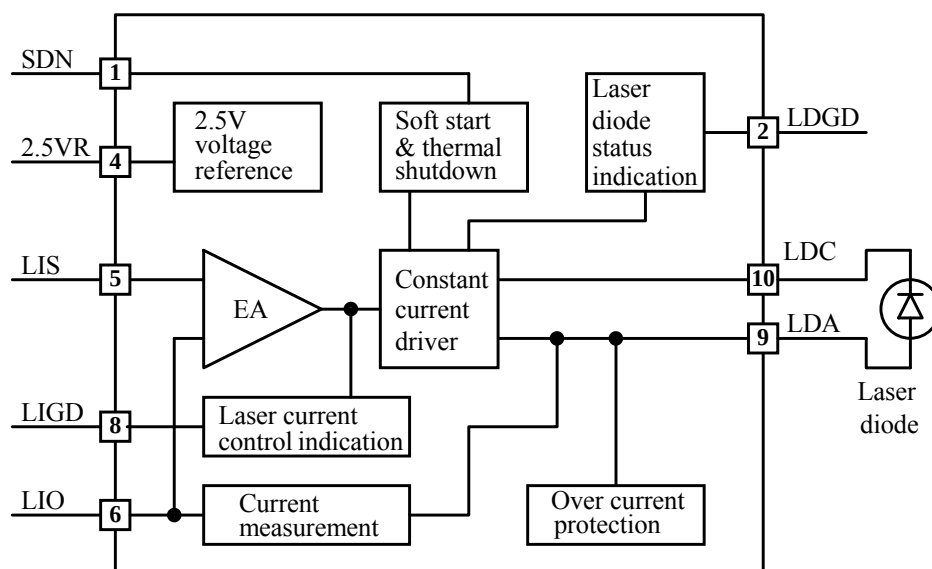
Figure 3. Block Diagram
