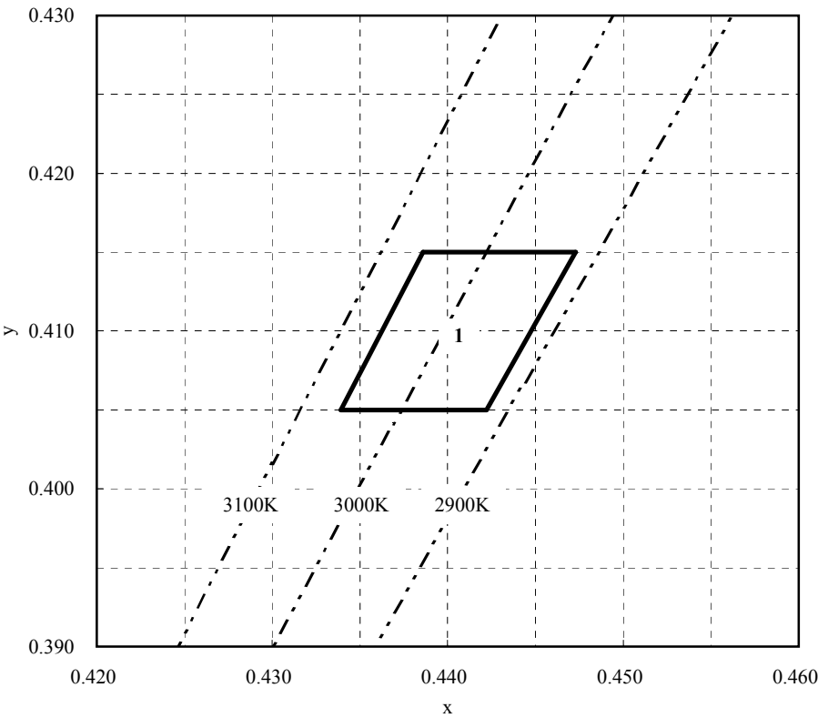
Chromaticity Diagram
