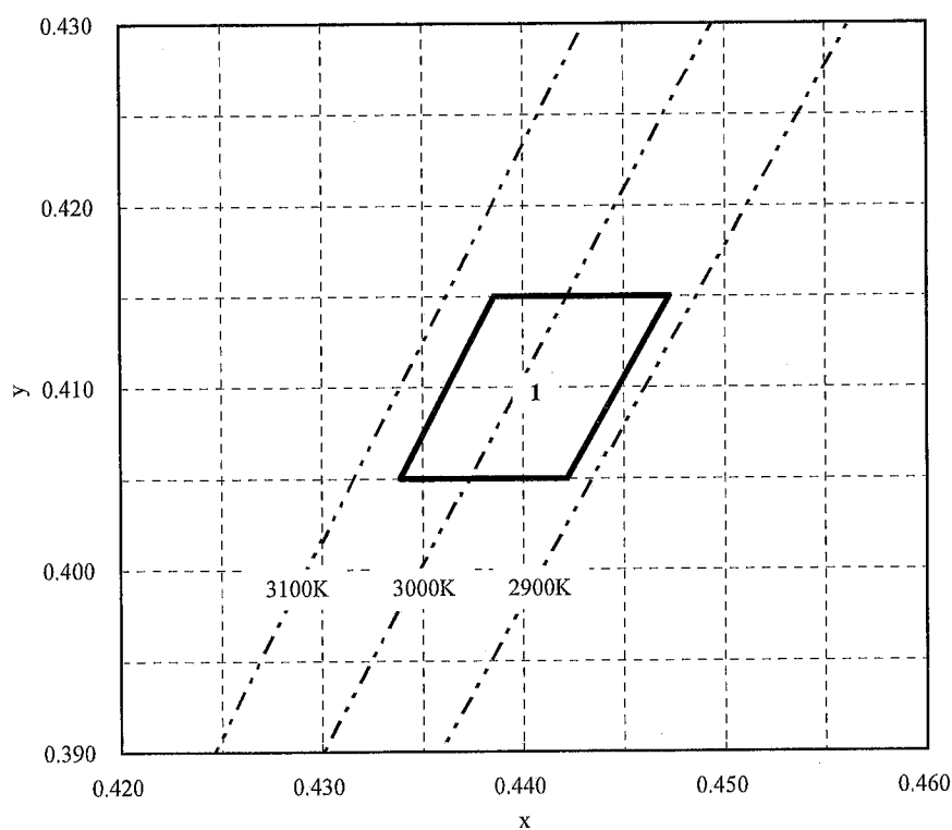
Chromaticity Diagram
