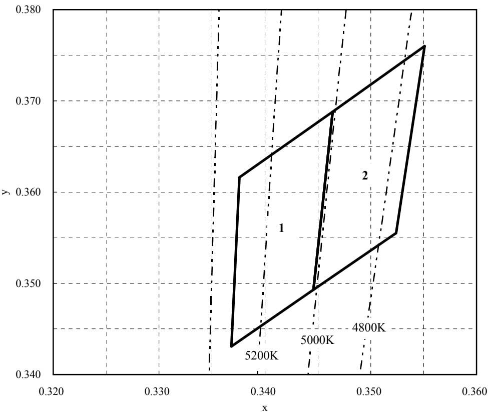
Chromaticity Diagram
