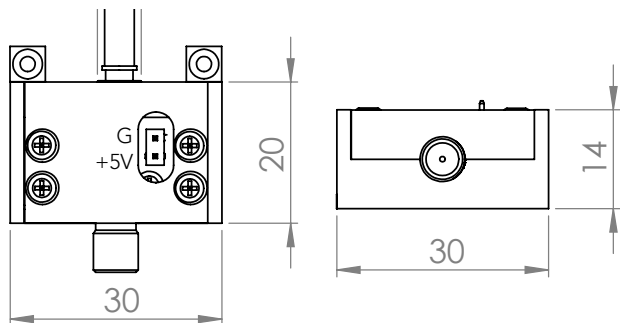
Mechanical Drawing of D-30 w/ External Housing 4
