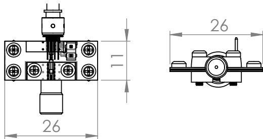
Mechanical Drawing of D-30 w/ External Housing 4
