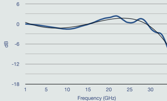
S21 O/E Response 1
