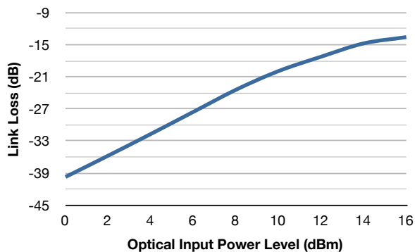
D-30 Link Loss
