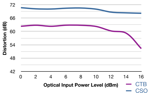
D-30 CSO, CTB Linearity Measurement 2
