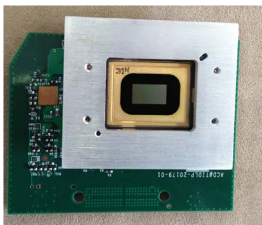
0.65" 1080p (1920x1080) DMD(A 封装)接口板
