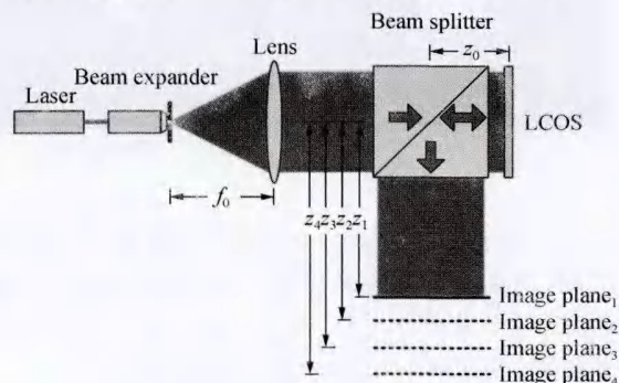
图 4 基于 LCOS 的多平面全息投影系统 Fig. 4 Scheme of multi-plane holographic projection system based on LCOS
