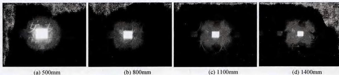
图 5 基于空分复用配置的全息投影结果图 Fig. 5 Holographic images captured on different planes with space division multiplexing configuration
